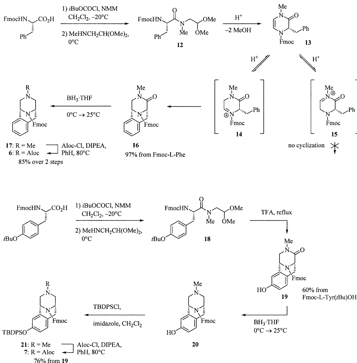
Scheme 1. Preparation of the iminobenzazocine scaffolds
