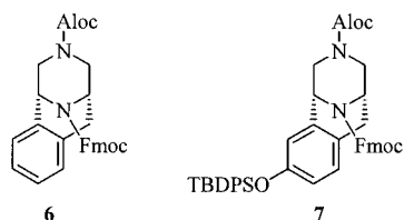
Figure 2. Selectively deprotectable iminobenzazocine scaffolds
