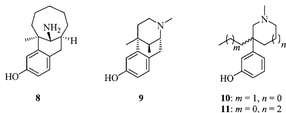
Figure 3. Opioid receptor ligands
